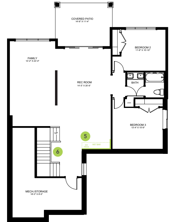
WALK-OUT FLOOR 1224 SQ FT
