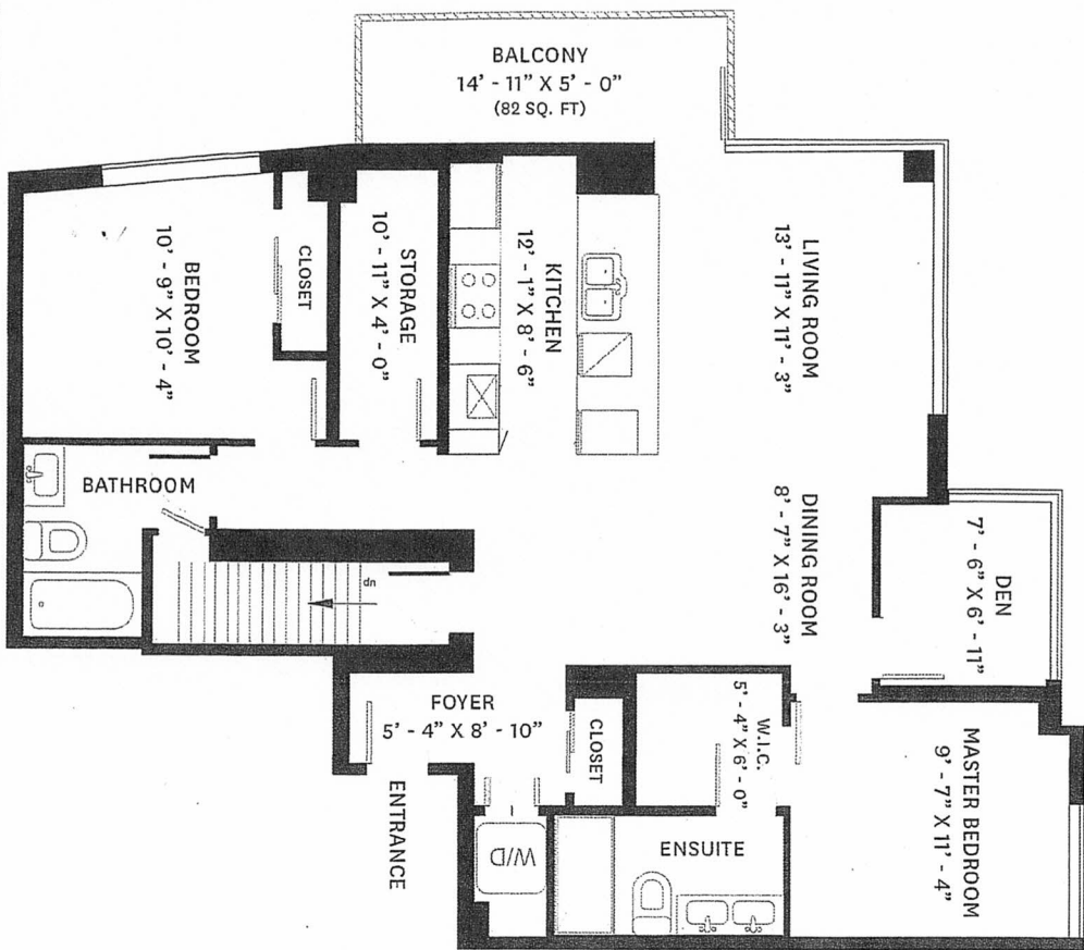
MAIN FLOOR PLAN Ceiling Height: 9' - 8"
