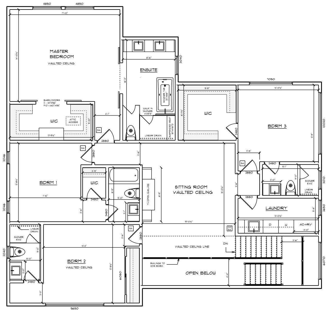
UPPER FLOOR PLAN CEILING HEIGHT = 108.75" SCALE: 1/4" = 1'-0" UPPER FLOOR = 1905.70 SQ FT
